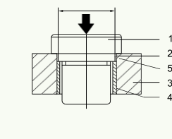
(b) 嵌入式安装 (B) Inset Installation
